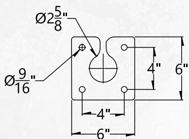
SUPPORTS BOLTING PATTERN
